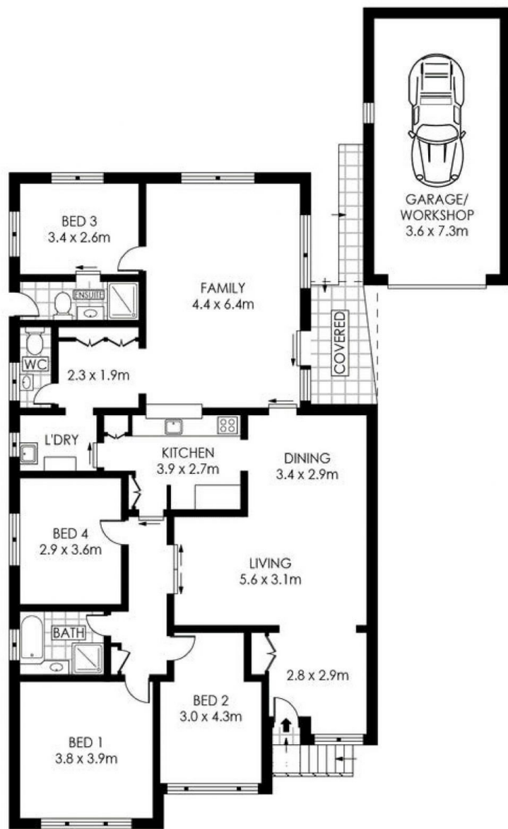
GROUND FLOOR
